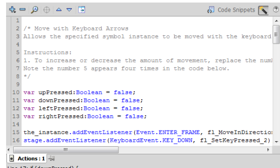
Figure 21 Actions panel
