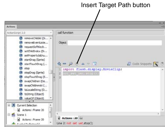
Figure 4 Stop method
