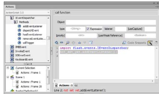
Figure 9 The addEventListener method in the Actions toolbox
