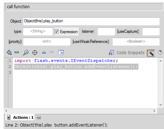
Figure 11 Event listener code in the Script pane
