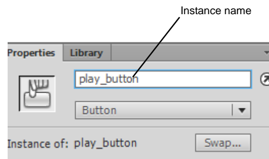
Figure 8 Button instance
