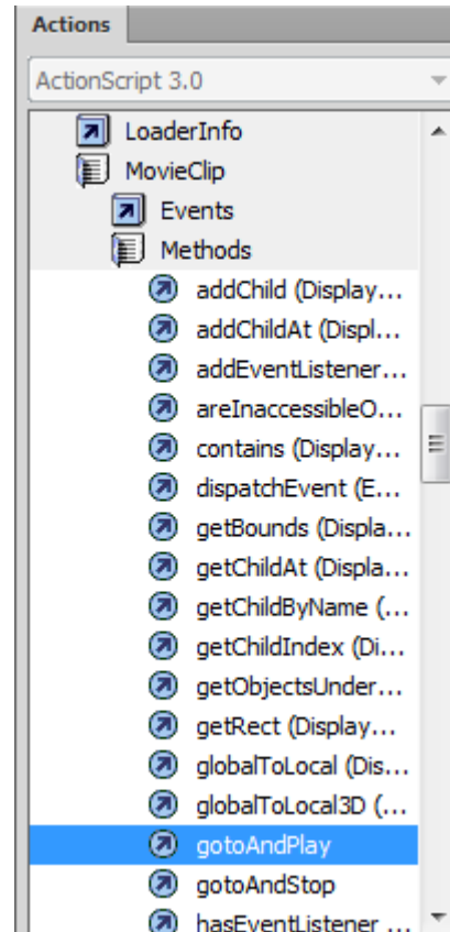
Figure 16 GotoAndPlay method
