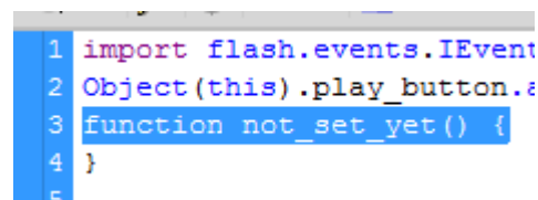
Figure 15 Function code
