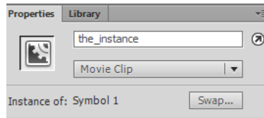
Figure 18 Properties panel.
