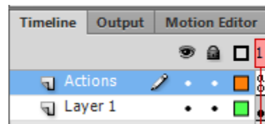
Figure 22 Timeline panel
