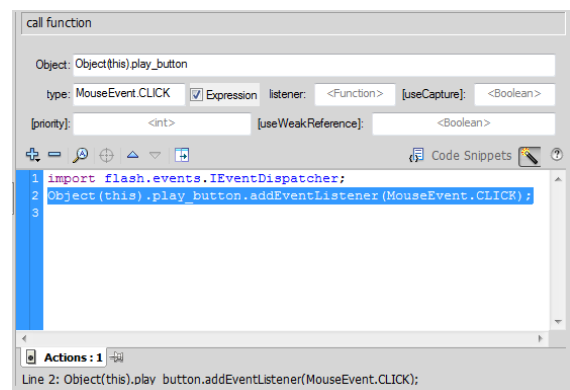
Figure 13 CLICK property in the Script pane
